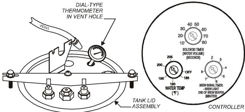
Fig. 13 Checking and Adjusting Brew Temperature
