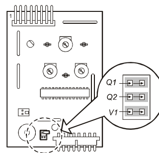
Fig. 18 Controller Jumpers
