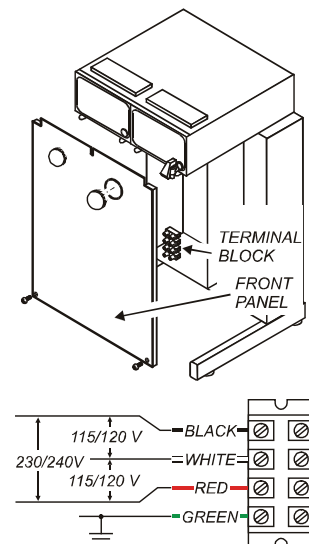
Fig. 3 115/240V Terminal Block
